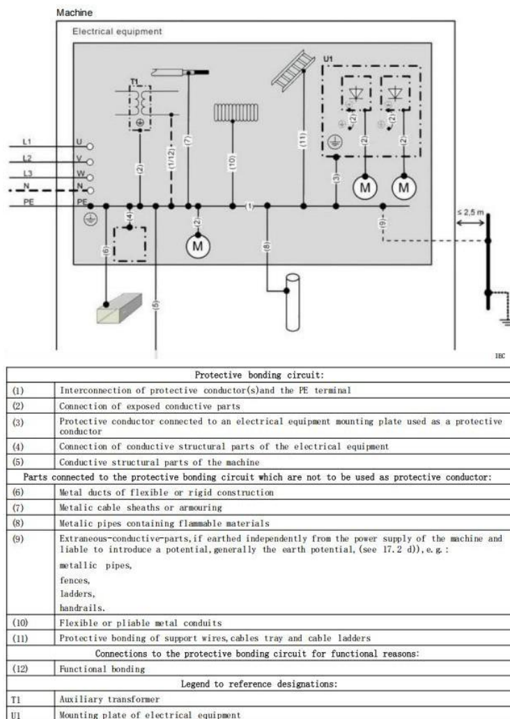
Figure 4-Example of equipotential bonding for electrical equipment of a machine
